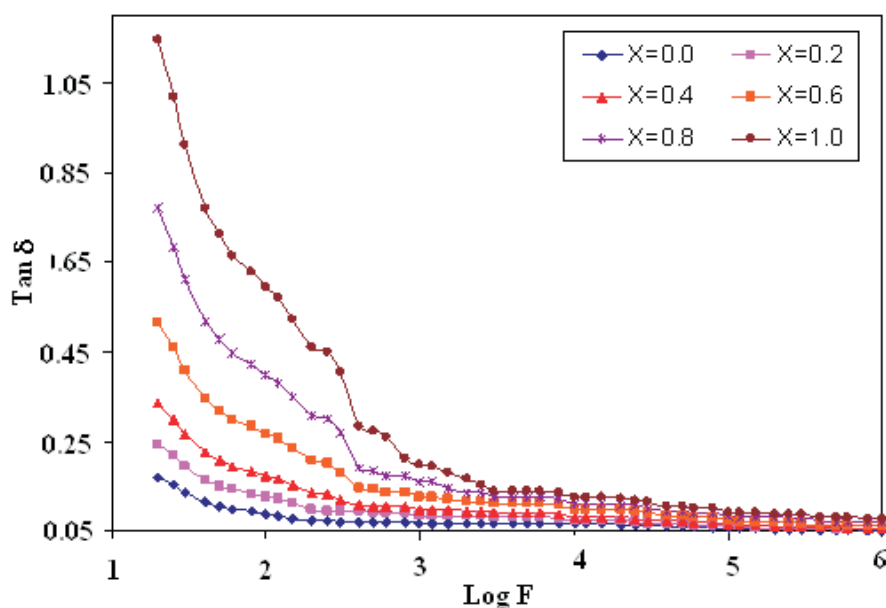
Fig. 3 Variation of dielectric loss tangent ( \tan \delta ) with frequency (F) for (1-x) \text{NiFe}_2\text{O}_4 + (x) \text{KNbO}_3
