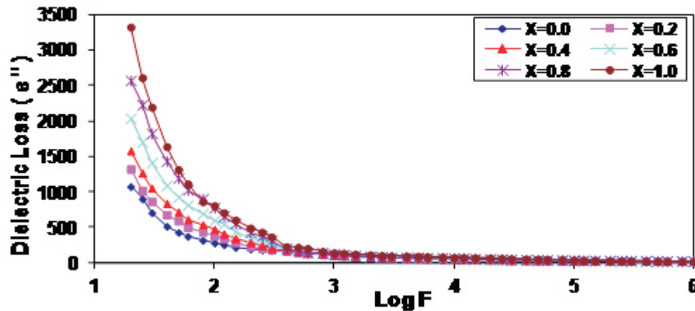
Fig.1 Variation of dielectric constant ( \epsilon' ) with frequency (F) for (1-x) \text{NiFe}_2\text{O}_4 + (x) \text{KNbO}_3 .
